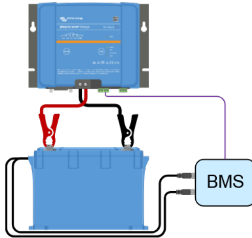
Initial charge using a BMS
