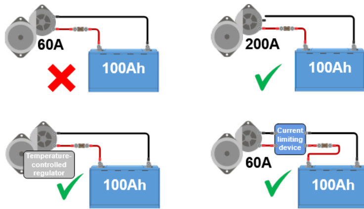
Alternator charging
