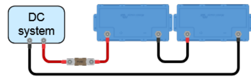
Multiple batteries in series
