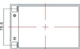
T30-1 Terminal
