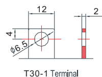
T30-1 Terminal
